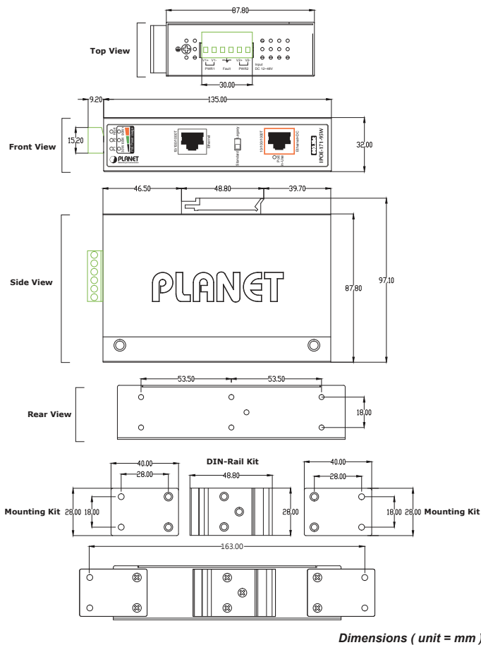
Figure 1: IPOE-171-95W dimensions
