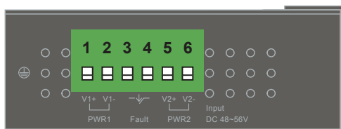
Figure 4: IPOE-171-60W upper panel.
