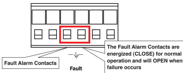
Figure 9: Fault Alarm Contact
