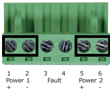
Figure 7: PWR1 & PWR2 Pins of Terminal Block.
