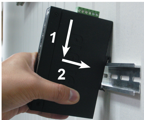
Figure 10: Mounting industrial device on DIN rail.
