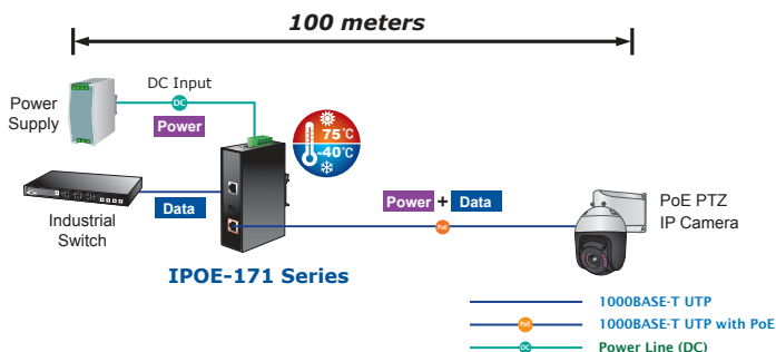
Figure 14: Connecting architecture with IEEE 802.3at/bt device
