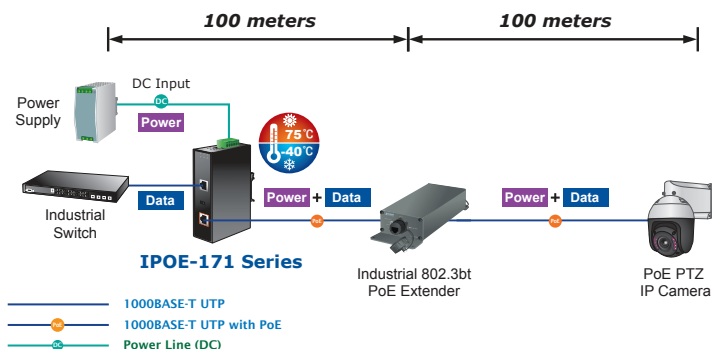
Figure 16: Connected Architecture of IPOE-171-60W and IPOE-E172
