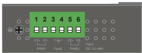
Figure 5: IPOE-171-95W upper panel.
