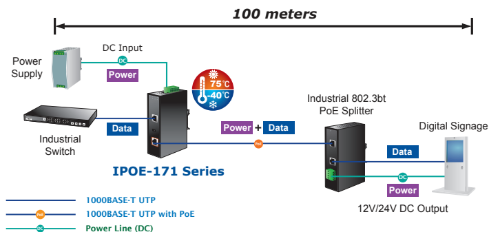
Figure 15: Connected Architecture of IPOE-171-60W and IPOE-171S
