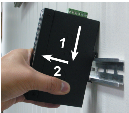
Figure 12: Removing industrial device from DIN rail
