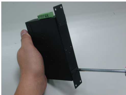
Figure 13: Attaching brackets to the industrial device.
