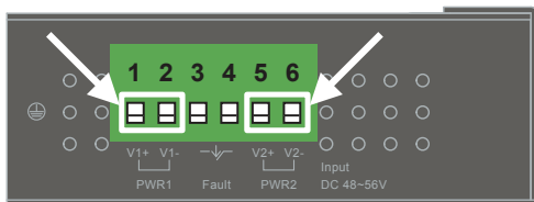
Figure 6: Power input pins.
